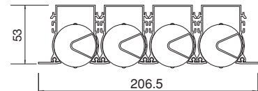
LD 140 No Flange : Overall Flange Dimensions
