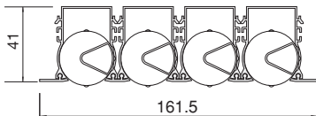
LD 130 No Flange : Overall Flange Dimensions
