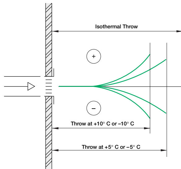
The Effect of Temperature on Free Space Jets
