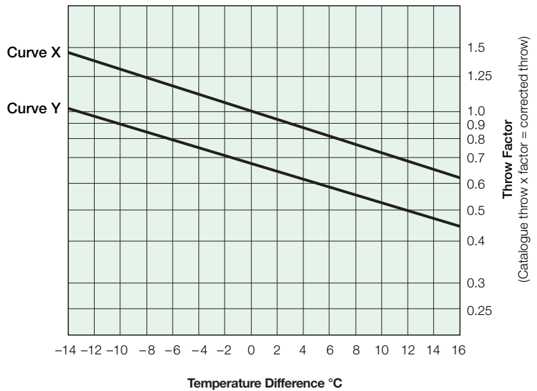
The Effect of Temperature on Vertical Discharge
